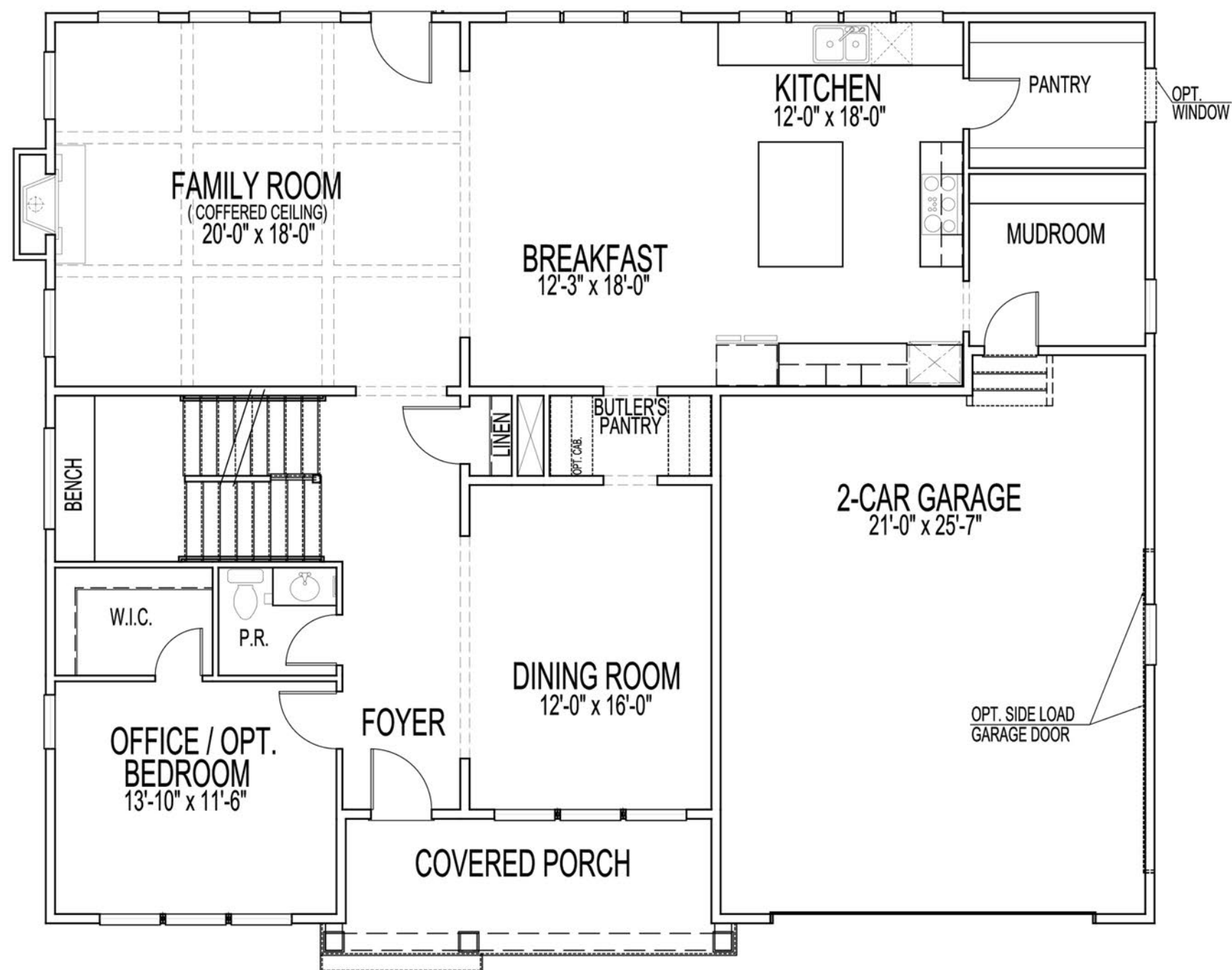
STANDARD FIRST FLOOR PLAN
