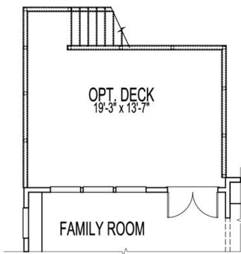
FIRST FLOOR PLAN W/ OPT. DECK
