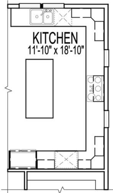
FIRST FLOOR PLAN W/ OPT. ALT. KITCHEN
