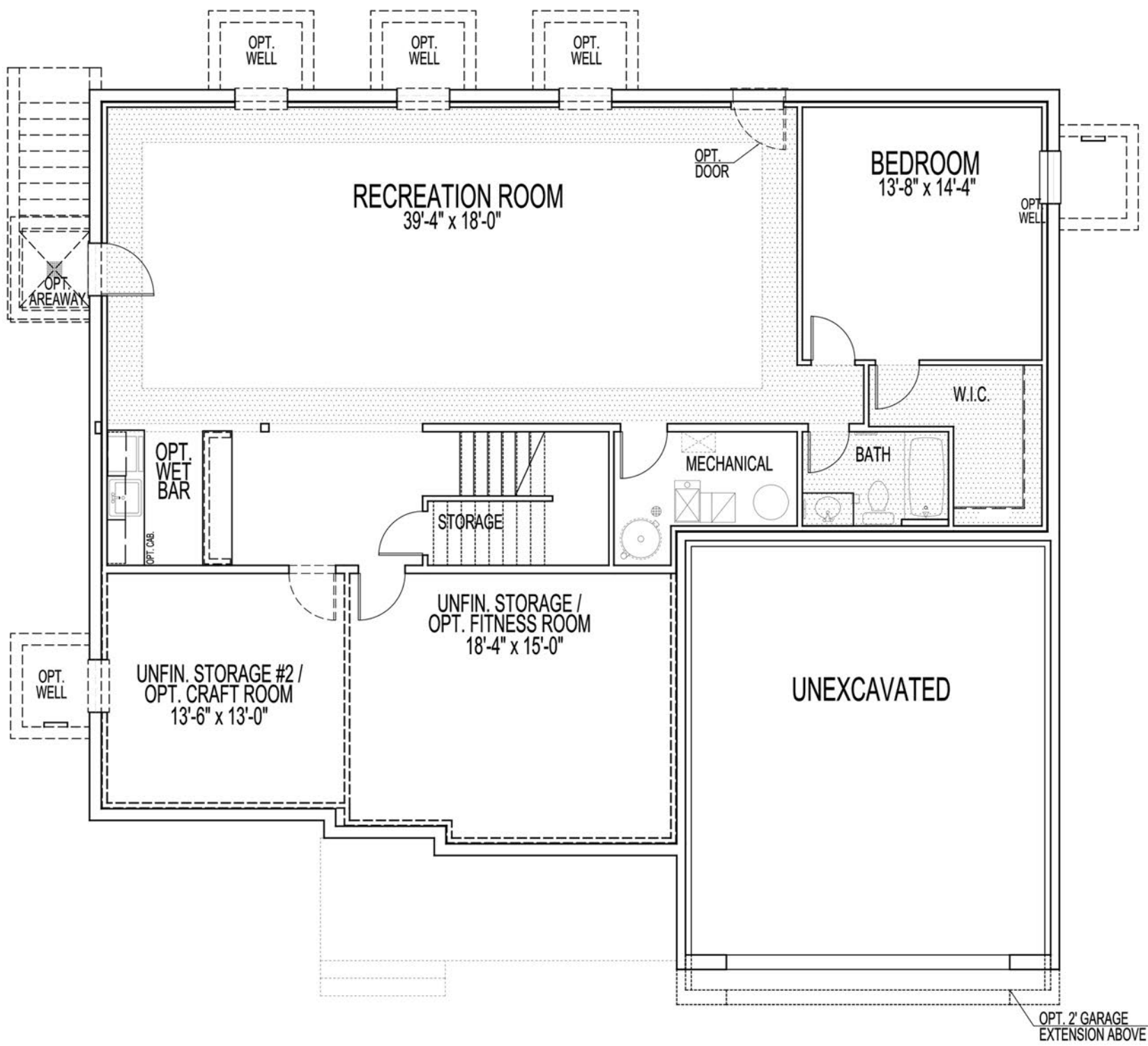
STANDARD BASEMENT FLOOR PLAN
