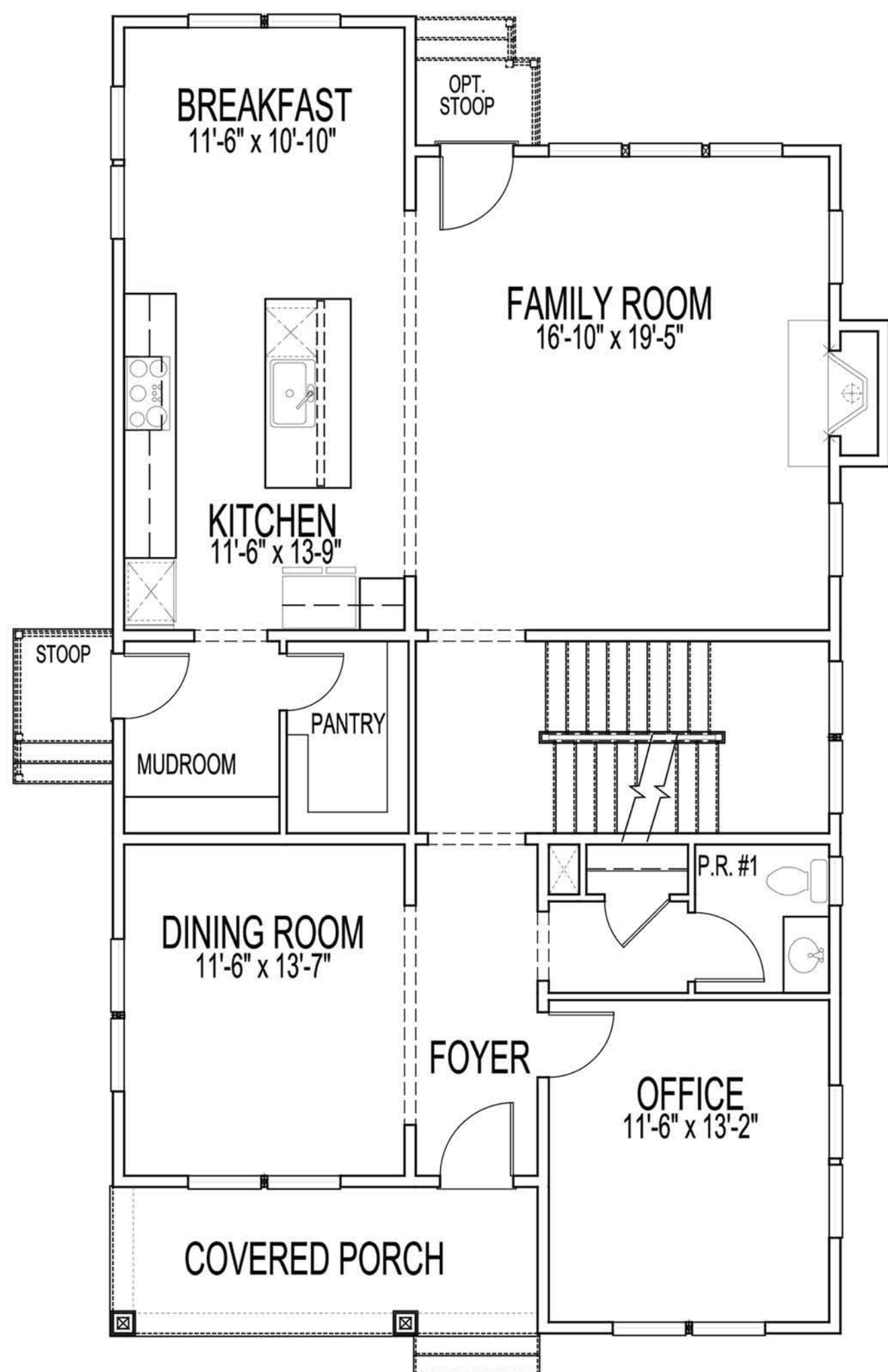
STANDARD FIRST FLOOR PLAN
