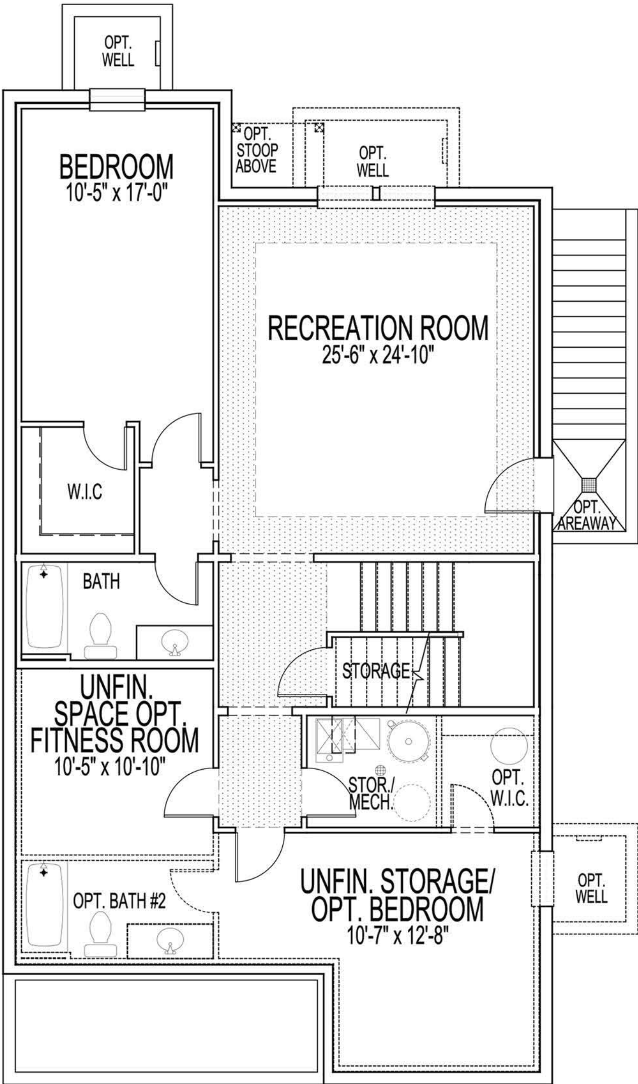
STANDARD BASEMENT FLOOR PLAN
