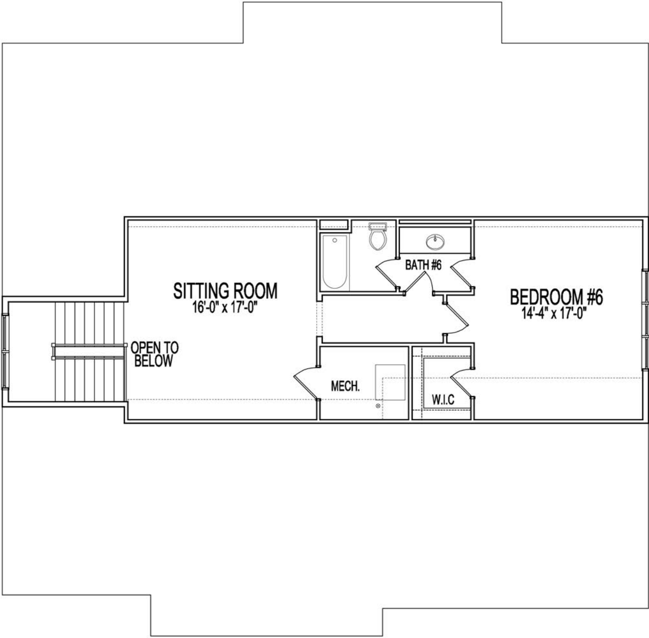
OPTIONAL ATTIC FLOOR PLAN
