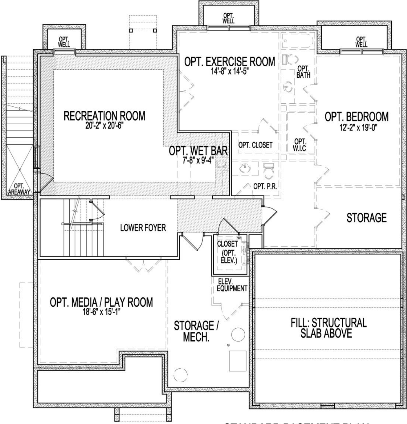
STANDARD BASEMENT PLAN
