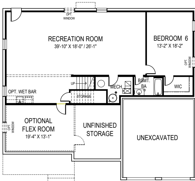
BASEMENT PLAN
