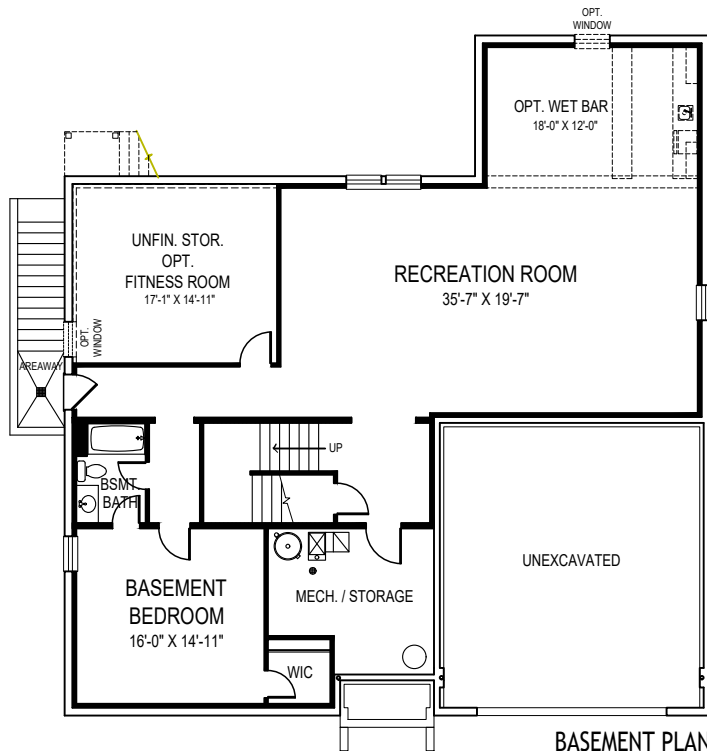
BASEMENT PLAN
