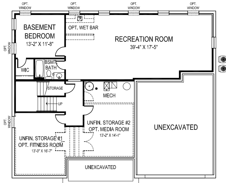
BASEMENT PLAN
