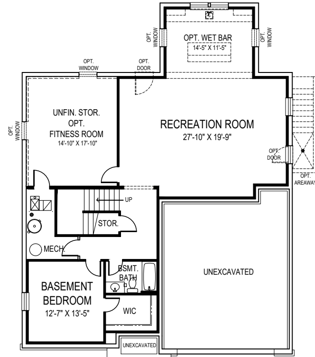
BASEMENT PLAN
