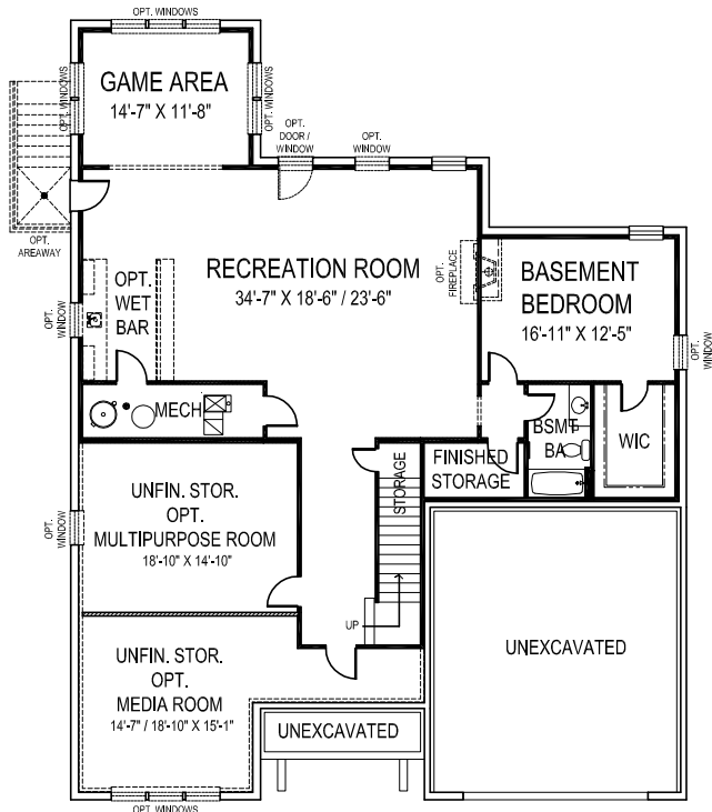
BASEMENT PLAN
