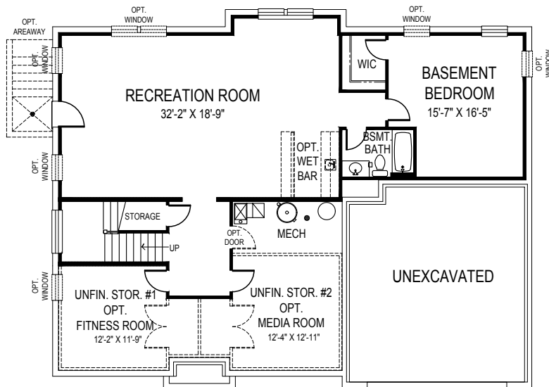
BASEMENT PLAN
