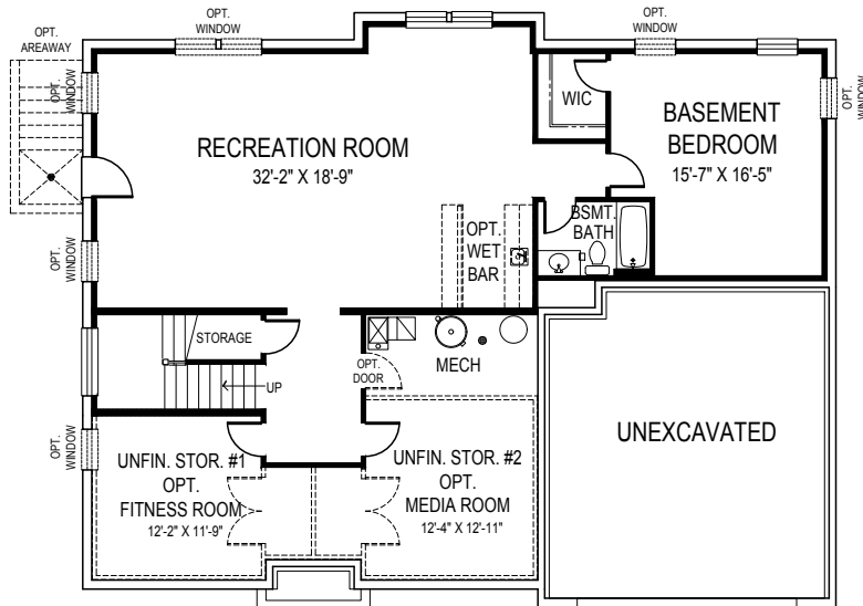
BASEMENT PLAN
