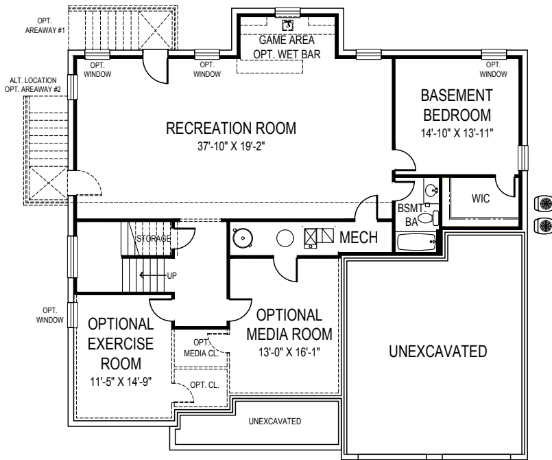
BASEMENT PLAN
