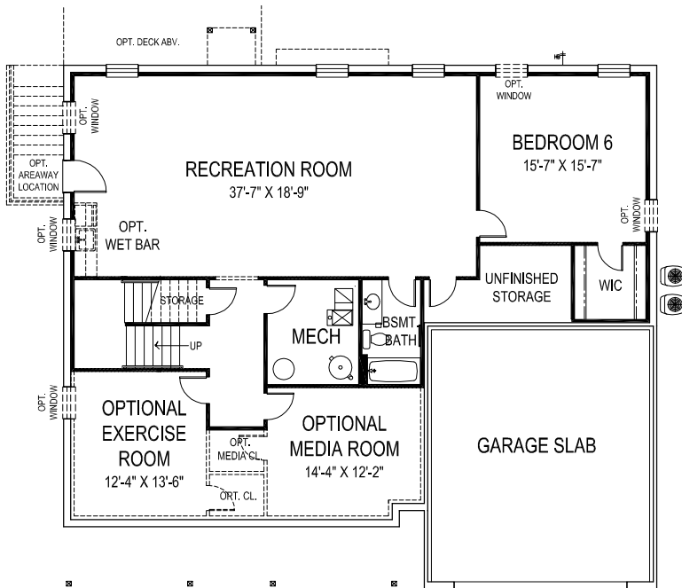
BASEMENT PLAN
